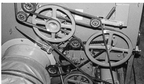
Dryer (V-belt)
