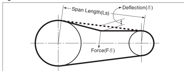
Fig. 3-3 Deflection measurement
