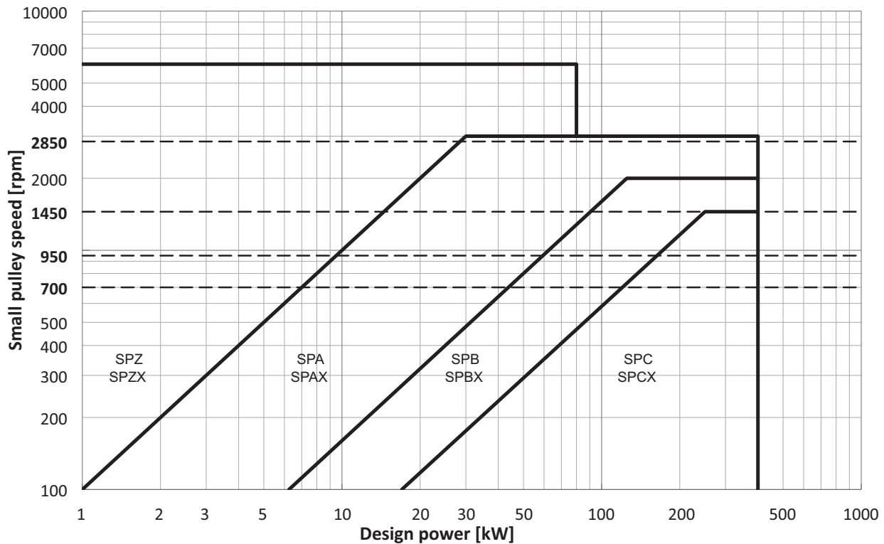
Cross section selection chart for Narrow V-belts
