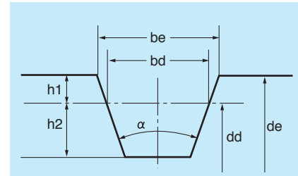
Fig. 3-2 Measuring pulley
