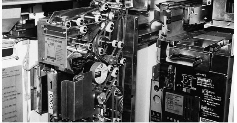
Prepaid-Kartenautomaten (Polyurethananer Zahnriemen)
