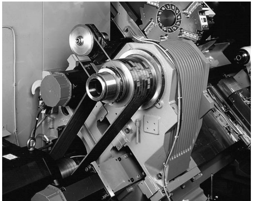
NC Drehbank (RIBSTAR Riemen)
